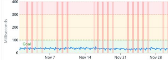
TTFB - Time To First Byte (P75)
